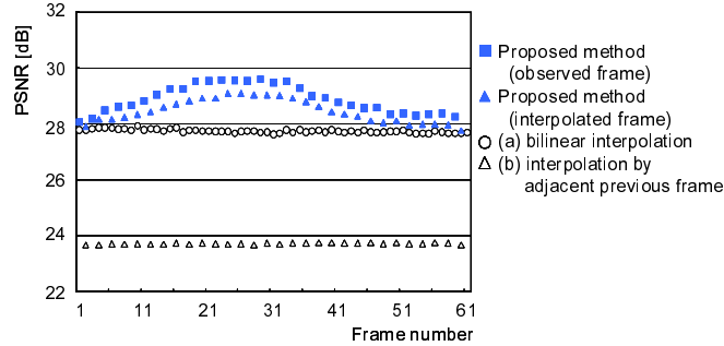
Fig. 6. Comparison of PSNR between the ground truth images and the images by each method
