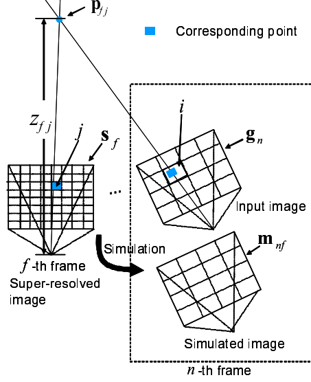
Fig. 1. Relationship between an input image and a super-resolved image
