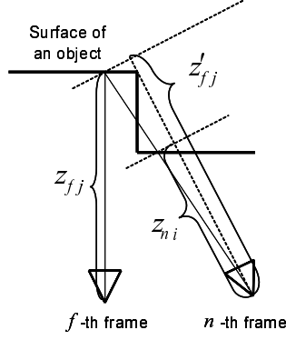
Fig. 2. Difference in depth by occlusion
