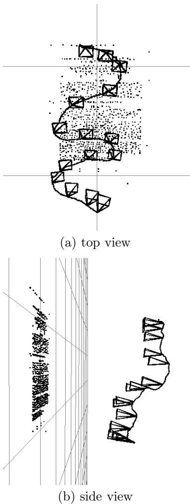
Figure 6. Estimated extrinsic camera parameters and feature positions (sequence 1).
