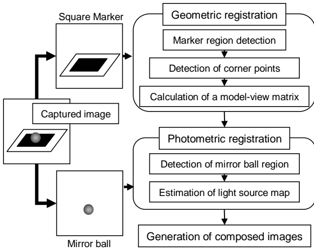
Figure 2. Flow diagram of the registration method.
